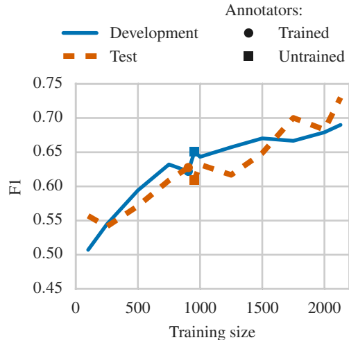
Figure 1: F_1 of predictions using an increasing number of training instances. • and ■ indicate models trained exclusively on labels from trained and untrained workers.
